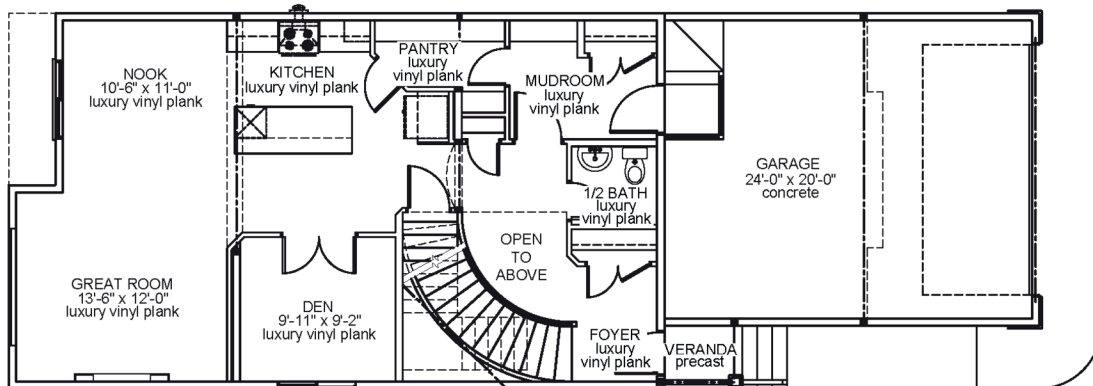
Main Floor Area: 975 sqft
