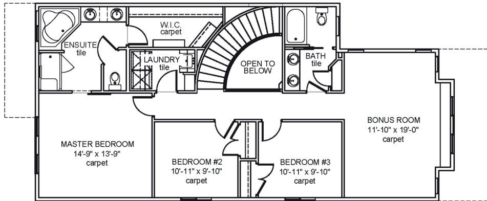
Upper Floor Area: 1228 sqft
