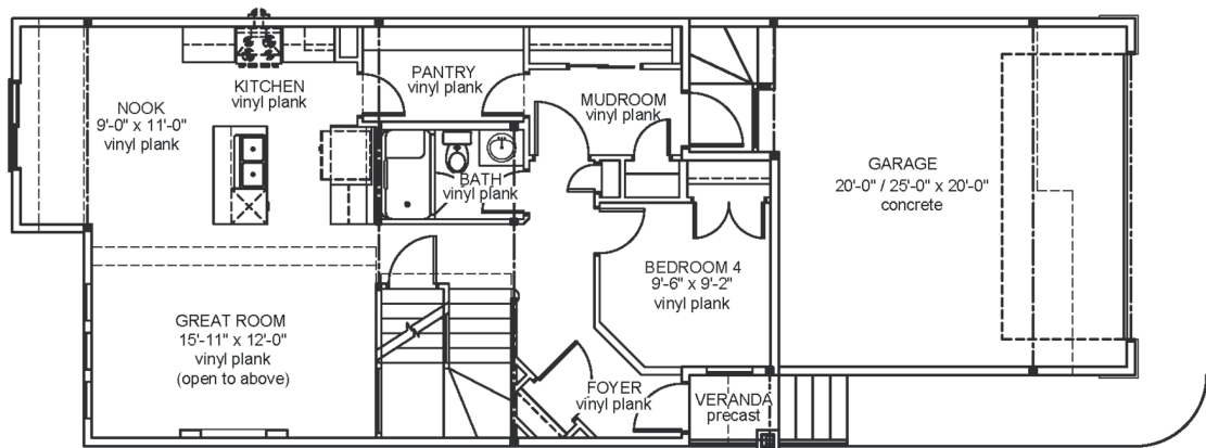
Main Floor Area: 926 sqft
