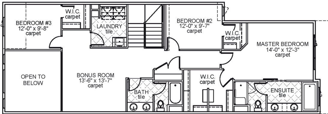
Upper Floor Area: 1308 sqft
