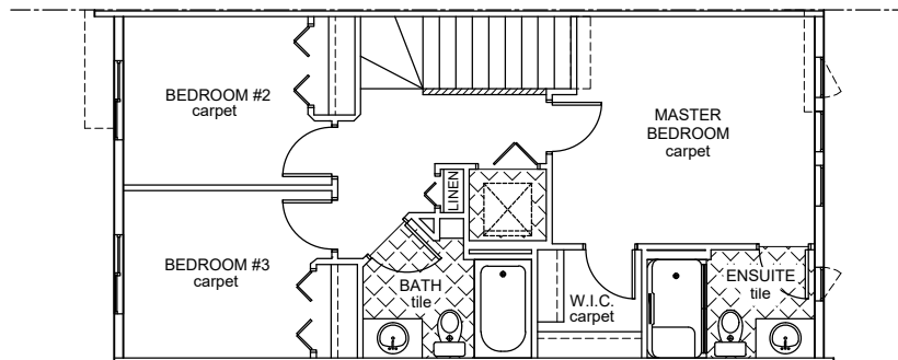
Upper Floor Area: 606 sqft
