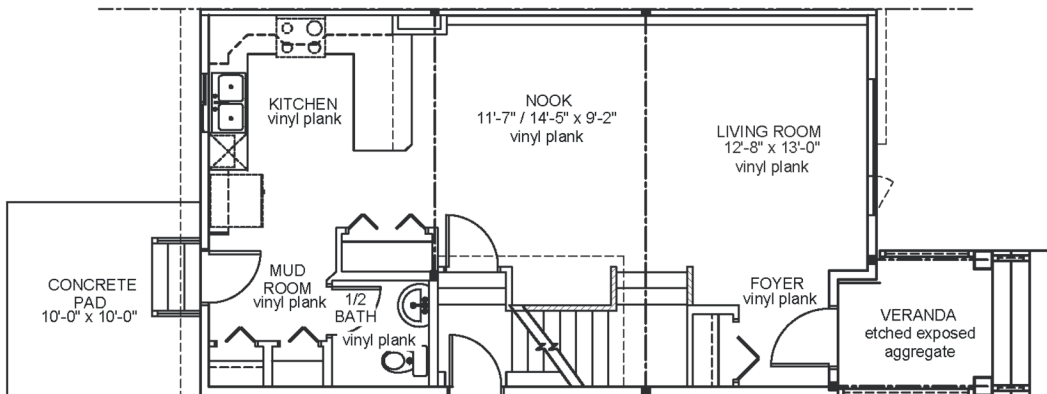
Main Floor Area: 687 sqft
