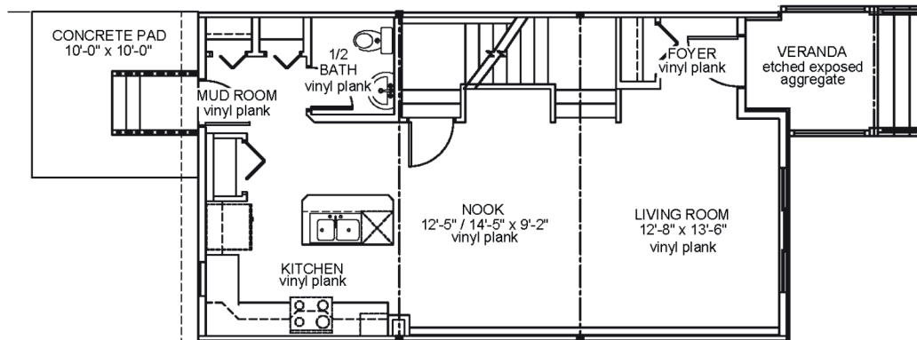
Main Floor Area: 692 sqft
