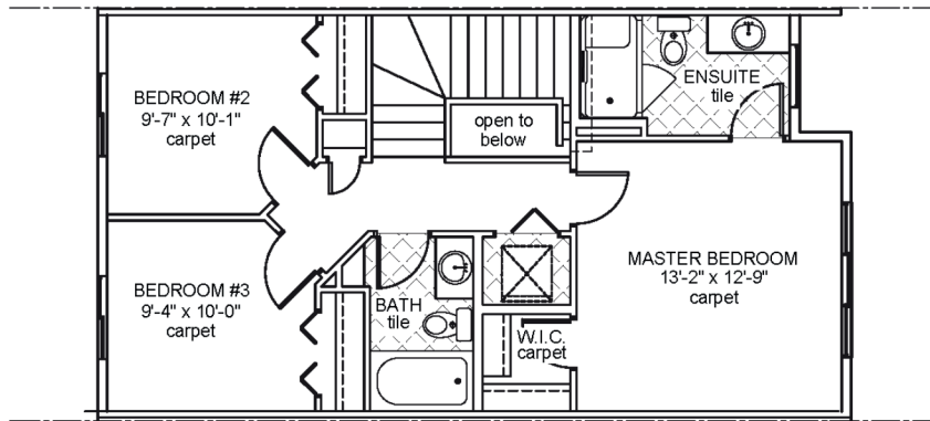
Upper Floor Area: 646 sqft
