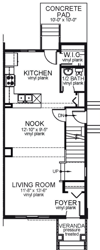
Main Floor Plan - 655 sq.ft. 9'-1" Main Floor Ceiling (Shown with Option #2)
