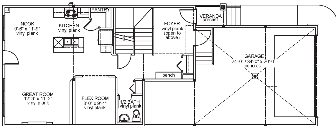
Main Floor Area: 822 sqft
