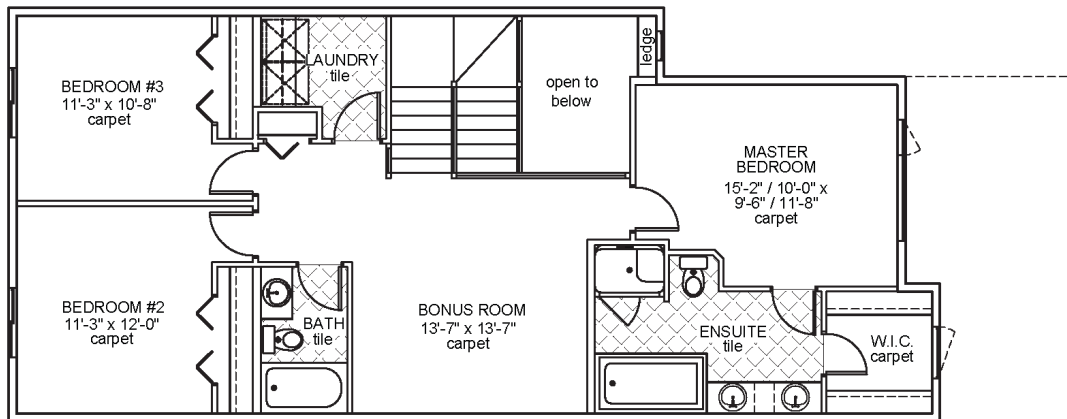
Upper Floor Area: 1076 sqft
