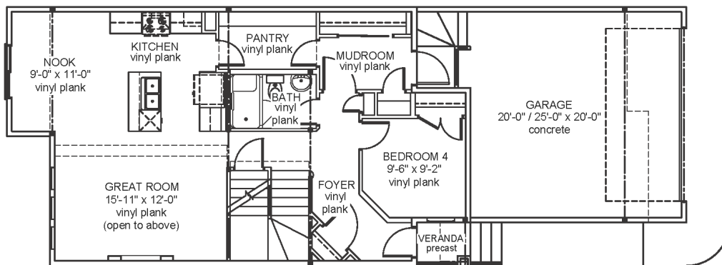
Main Floor Area: 926 sqft
