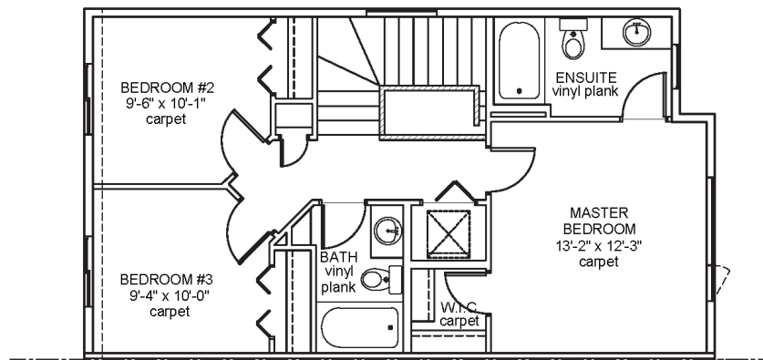
Upper Floor Area: 603 sqft
