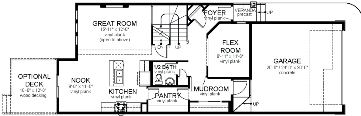
Main Floor Plan Area: 914 SQ. FT. 9'-1" Main Floor Ceiling (shown with Avanti Specifications)
