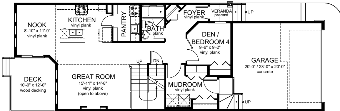
Main Floor Plan - 1,003 sq.ft. 9'-1" Main Floor Ceiling (Shown with Avanti Specifications)
