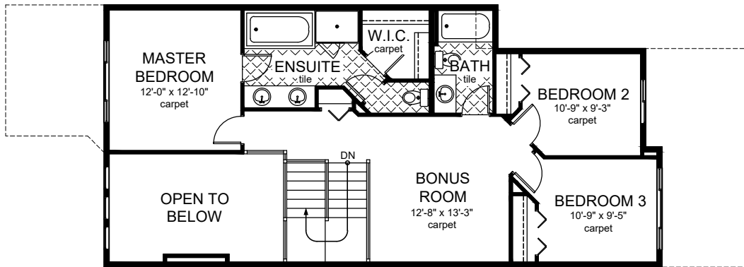
Upper Floor Plan - 923 sq.ft. (Shown with Avanti Specifications)
