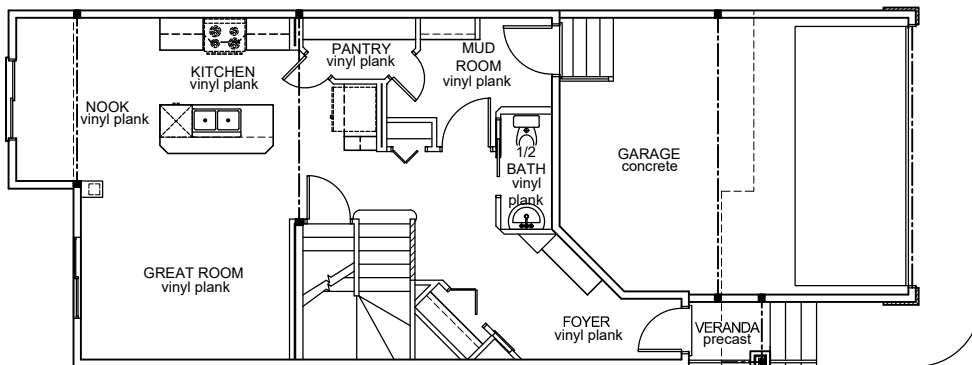
Main Floor Area: 749 sqft
