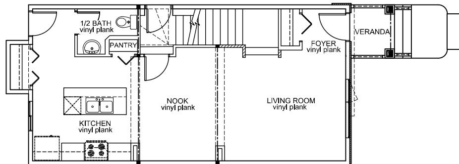
Main Floor Area: 663 ft 2
