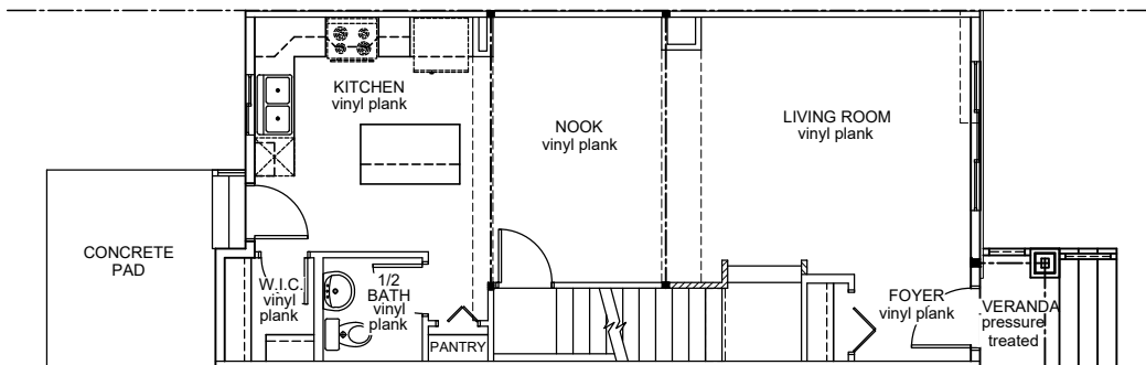
Main Floor Area: 672 sqft
