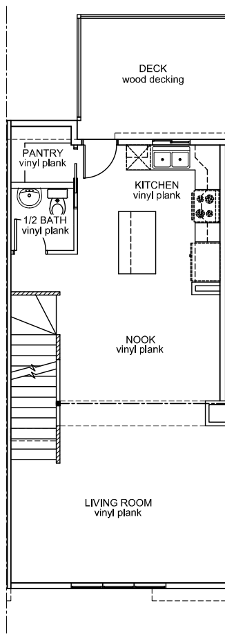
Main Floor Area: 657 sqft
