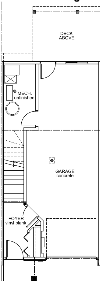
Ground Floor Area: 131 sqft
