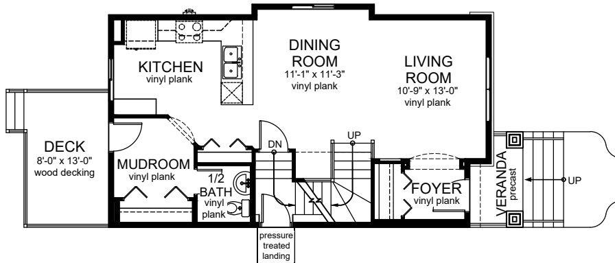
Main Floor Plan - 719 sq.ft. 9'-1" Main Floor Ceiling (Shown with Avanti Specifications, Corner Lot Treatment & Side Entrance)
